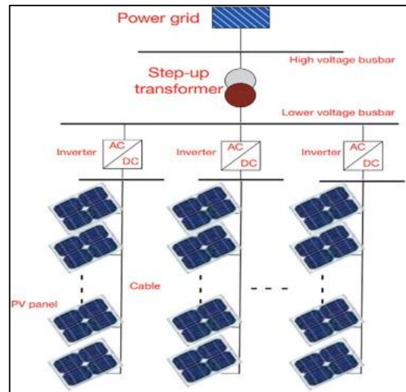
Figure 2: Diagram of a PV power station
